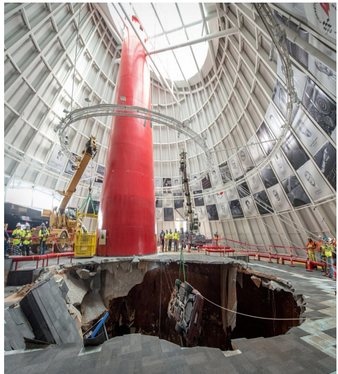
Figure 2, Collapse at Corvette Museum Skydome
