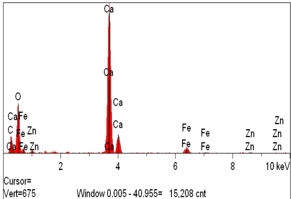
Figure 30: Analysis report for SEM image obtained for iron-coated limestone treated with zinc.
