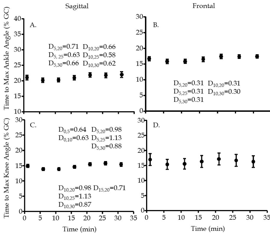
Figure 5A-D. The time it took to reach the maximum angles (Mean and standard error of the mean) during stance for the ankle (A, B) and knee (C, D) in the sagittal (A, C) and frontal (B, D) planes across the 31-minute run. Greater than moderate effect sizes of pairwise comparisons were reported here only if the outcome variable exhibited significant changes with time (A-C).
